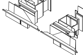
End cap for sash inversion profile S67758
